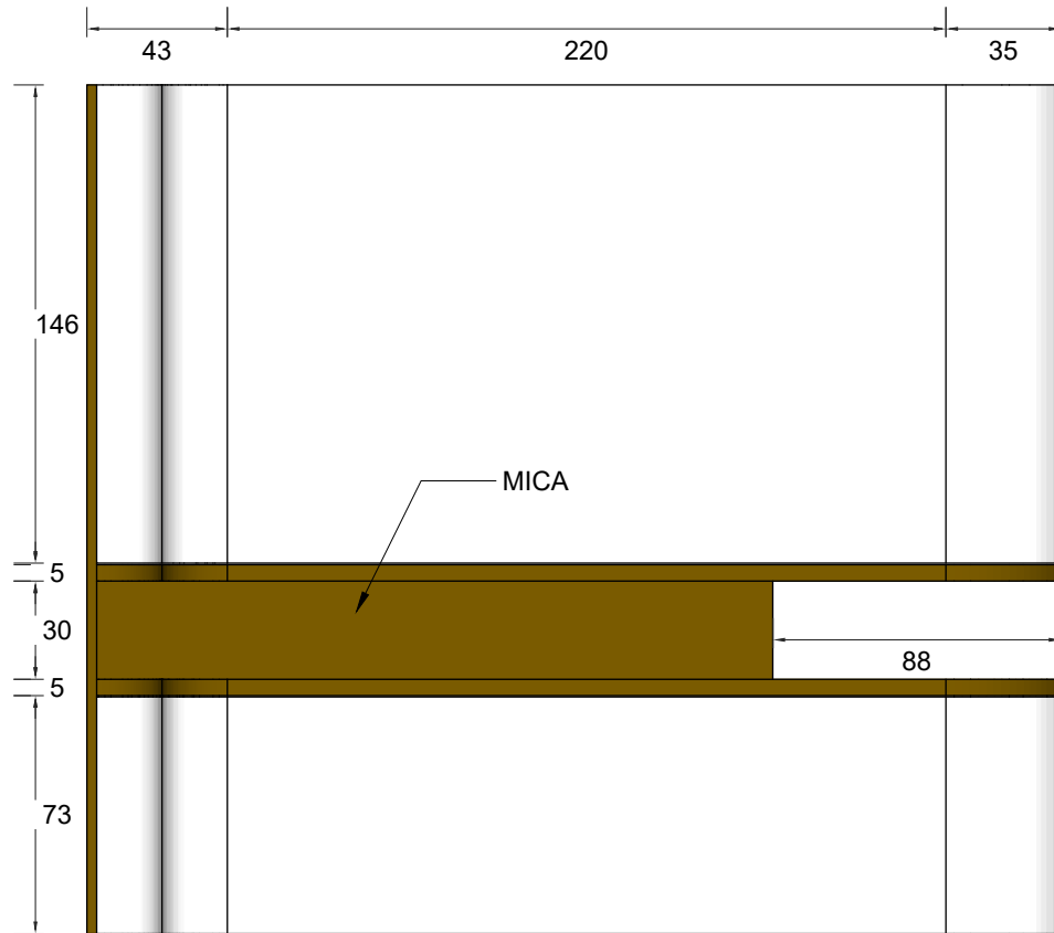
FRONT ELEVATION
